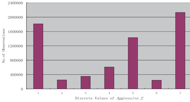
Figure 2. Distribution of Aggressive_2.
