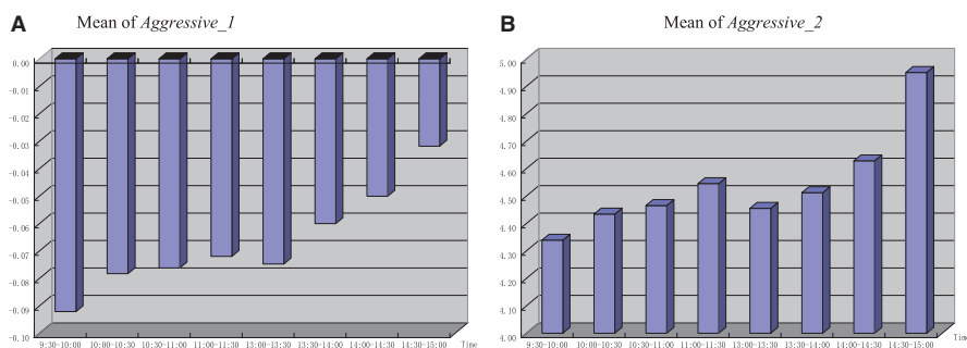
Figure 1. Aggressiveness measure variations during the course of a trading day.
