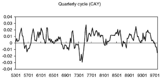
Fig. 2. Time series of three conditioning variables. Cycle (IP) is the cyclical element in monthly Hodrick–Prescott (1997) filtered industrial production. Cycle (GNP) is the cyclical element in quarterly Hodrick–Prescott (1997) filtered GNP. Cycle (CAY) is the aggregate consumption–wealth ratio, derived in Lettau and Ludvigson (2001a). Monthly data for IP are from 1952:01 to 1997:12. Quarterly data for GNP are from 1952:01 to 1997:04, and quarterly data for CAY are from 1953:01 to 1997:04.
