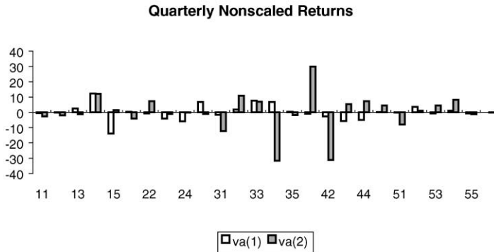
Fig. 1. Standardized eigenvectors of two largest eigenvalues of the weighting matrix W_T = [(1/T)\sum RR']^{-1} . The data are monthly and quarterly excess returns of the Fama-French 25 portfolios and the return on the T-bill. Monthly data are from 1952:01 to 1997:12. Quarterly data are from 1953:01 to 1997:04. The portfolio numbers on the x-axis are numbered ij with i indexing size increasing from one to five and j indexing book-to-market ratio increasing from one to five. The vector va(1) and va(2) are the eigenvectors corresponding to the two largest eigenvalues of W_T .
